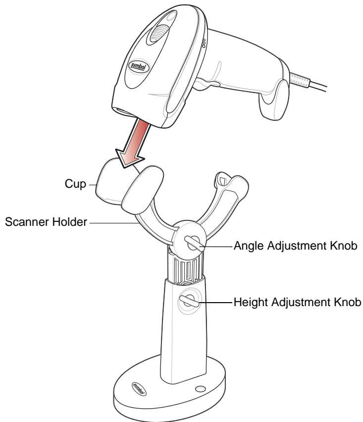
Figure 2-7 Inserting the Scanner in the Intellistand
