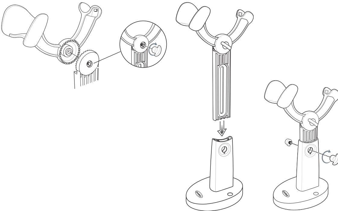
Figure 2-6 Assembling Intellistand
