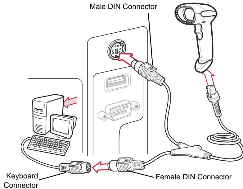
Figure 5-1 Keyboard Wedge Connection with Y-cable
