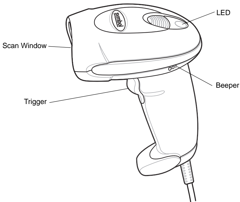
Figure 2-1 Parts
