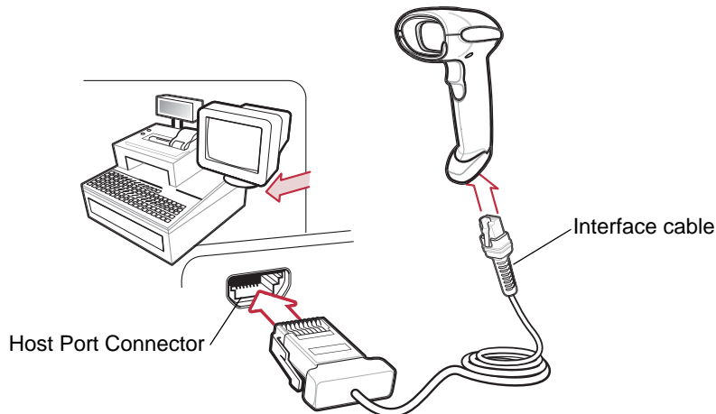
Figure 8-1 IBM Direct Connection
