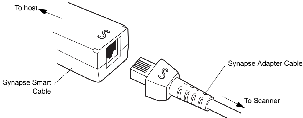
Figure 1-3 Synapse Cable Connection
