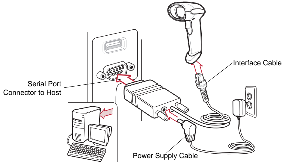
Figure 6-1 RS-232 Direct Connection
