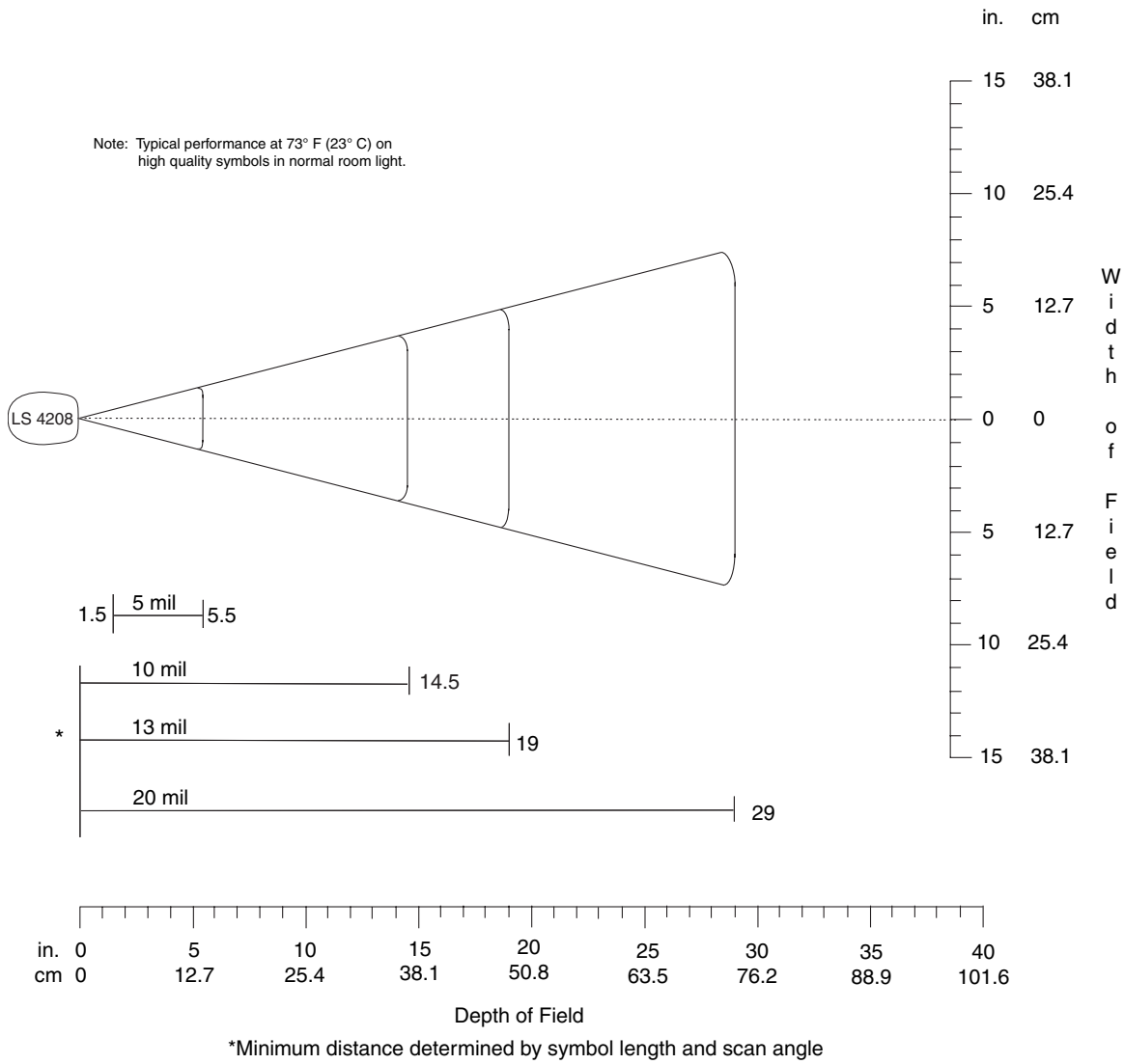
Figure 2-8 Symbol LS3008 Decode Zone
