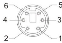
DIN 6 Female Pin Assignment.
