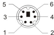
DIN 6 Male Pin Assignment.
