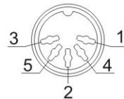
DIN 5 Female Pin Assignment.
