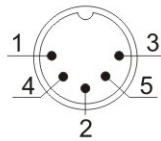
DIN 5 Male Pin Assignment.
